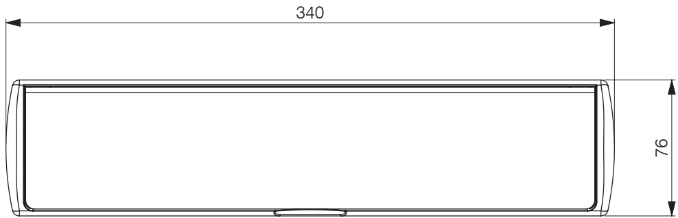
Internal Letterplate
